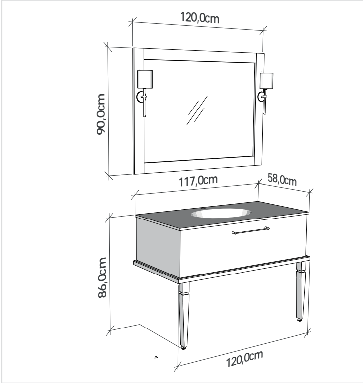
TRACE 120 cm Aplik aydınlatmalı ayna. Mirror with applique illumination.
